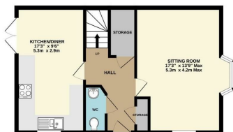
GROUND FLOOR 500 sq.ft. (46.4 sq.m.) approx.
